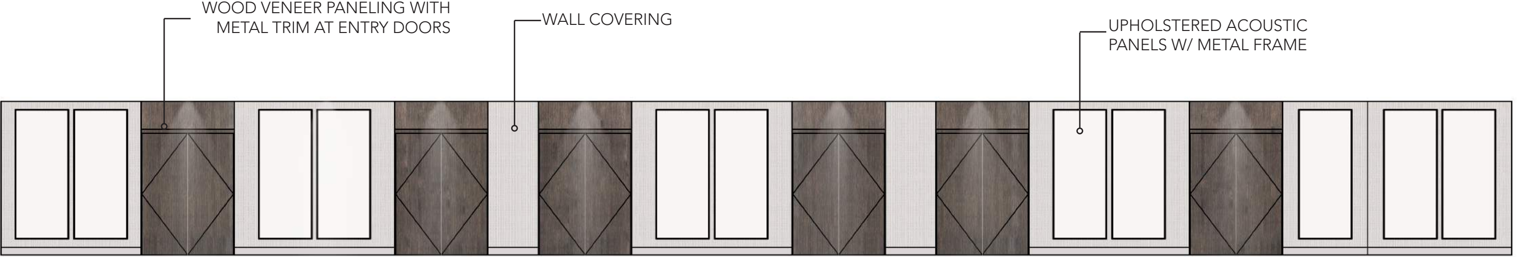
A - INTERIOR ENTRY WALL ELEVATION
