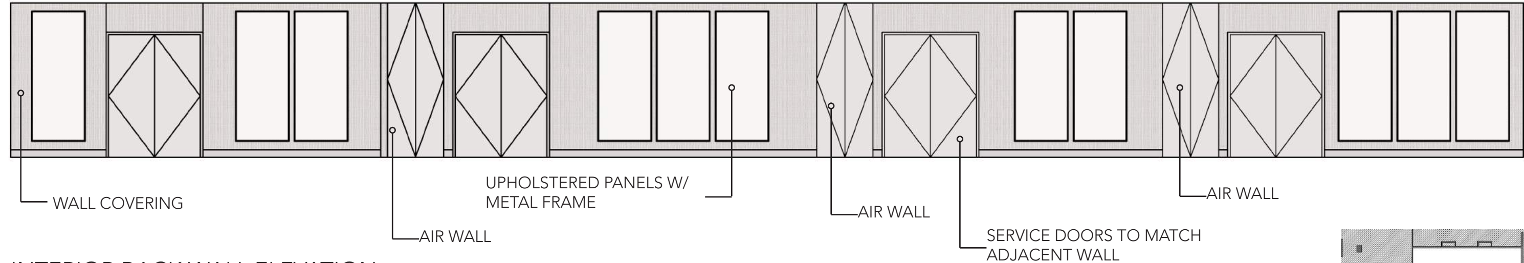
B - INTERIOR BACK WALL ELEVATION
