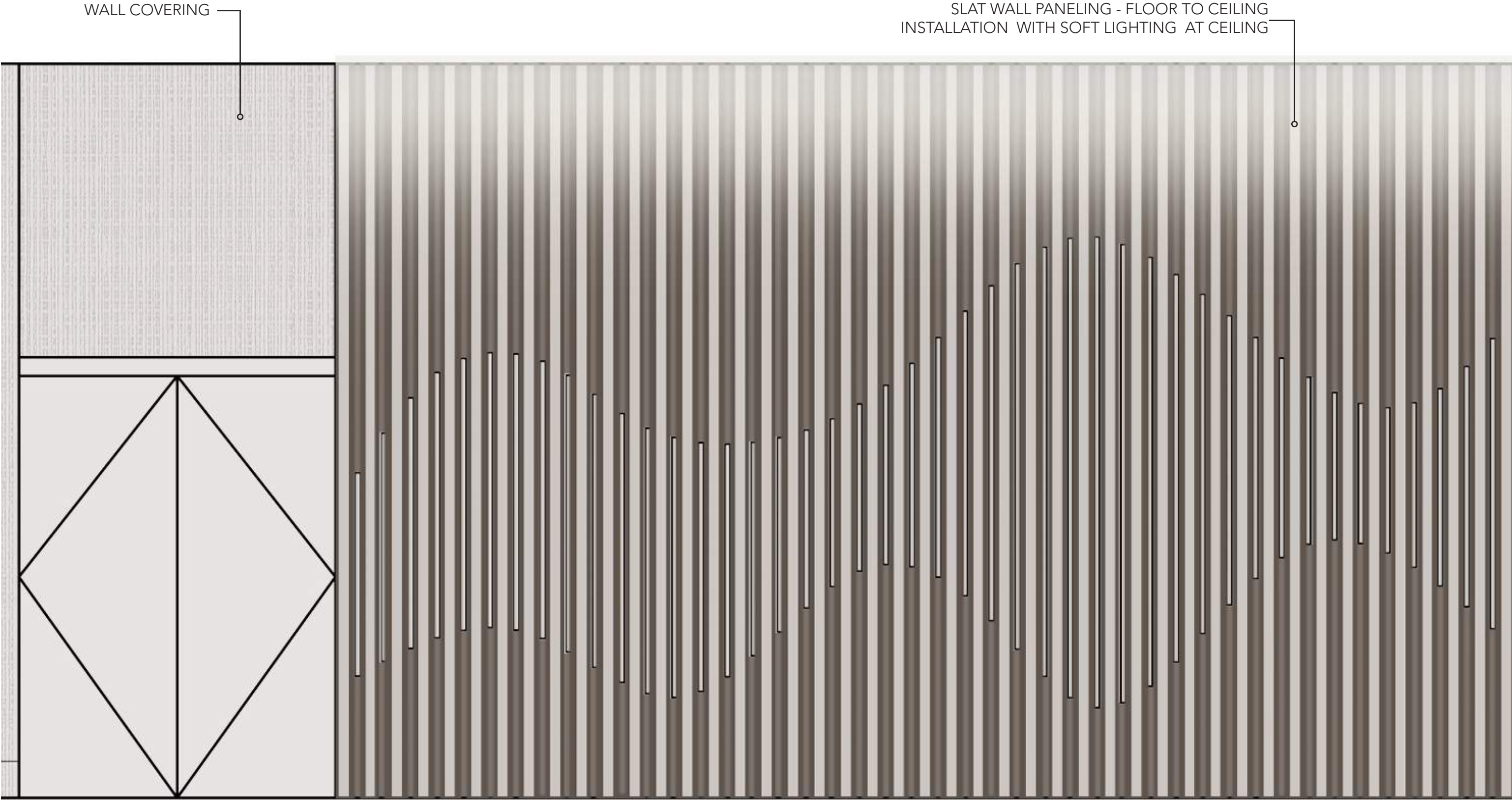
C - INTERIOR SIDE WALL ELEVATION CLOSE UP DETAIL
